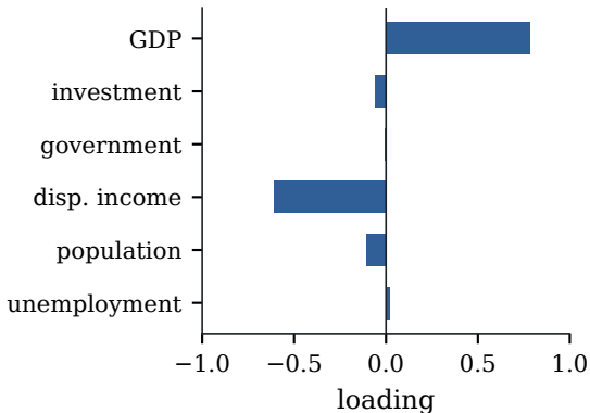
(b) smallest right singular vector
