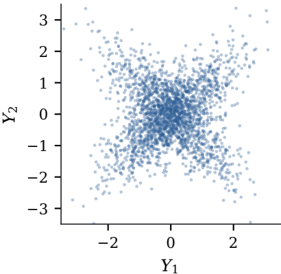
(a) normal marginals, zero correlation
