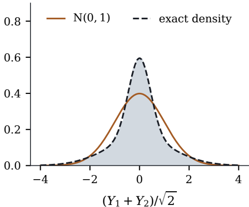
(b) a linear combination
