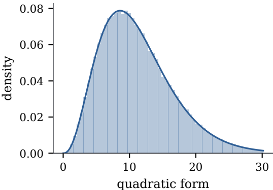
(a) GLS-centred: \chi^2(7, 4.20)
