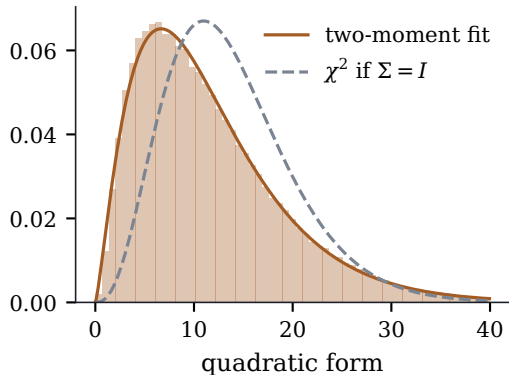
(b) ordinary centring
