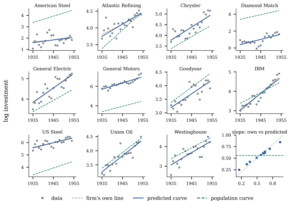
Figure 33.5.1: Log gross investment of eleven firms, 1935–1954, with each firm's own least squares line (dotted), its predicted curve \mathbf{X}(\hat{\beta} + \hat{u}_i) (solid) and the population curve \mathbf{X}\hat{\beta} (dashed). The last panel plots own slope against predicted slope.
