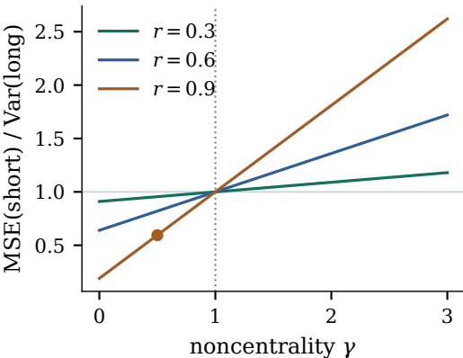
(a) omitting x_2 : estimating \beta_1
