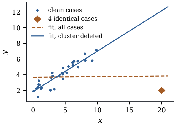
(a) data and two fits
