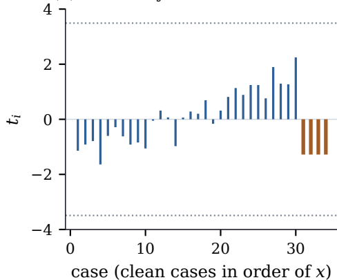
(b) externally studentized residuals
