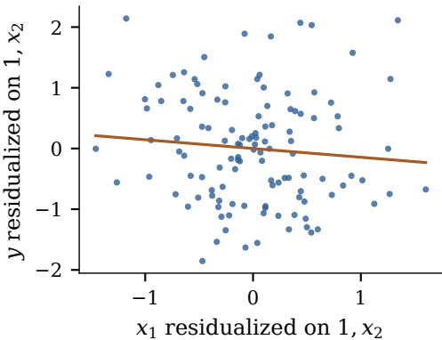
(a) added-variable plot
