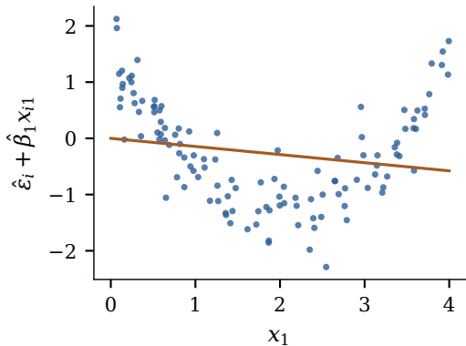
(b) component-plus-residual plot
