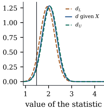
(c) null densities, n = 40
