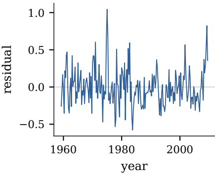
(a) residuals in time order
