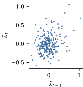
(b) lag plot, r_1 = 0.30
