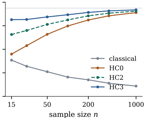
(b) sd proportional to x
