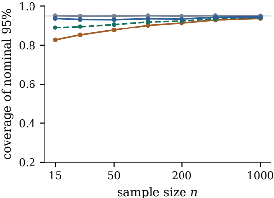
(a) constant variance
