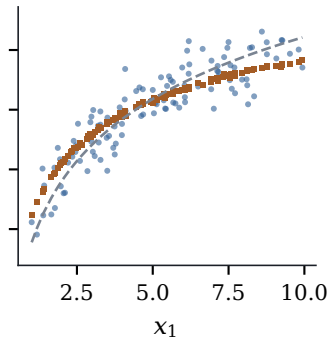
(c) (b), augmented
