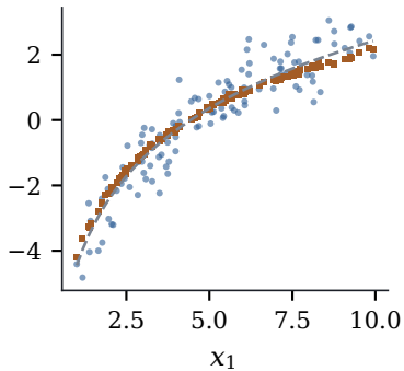
(a) x_2 linear in x_1
