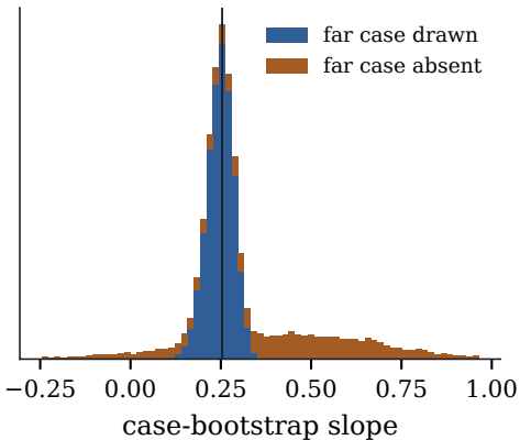
(a) one high-leverage case
