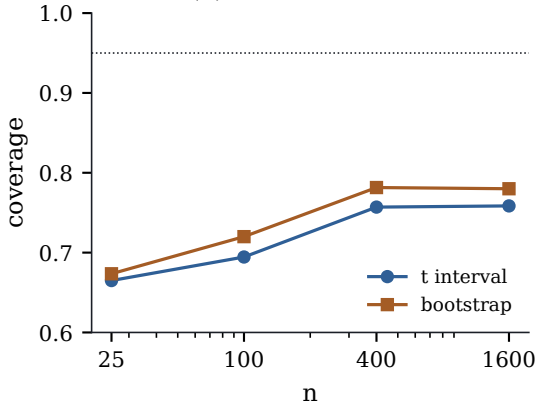
(b) infinite variance
