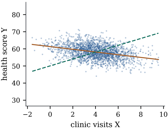
(a) observed: X follows illness
