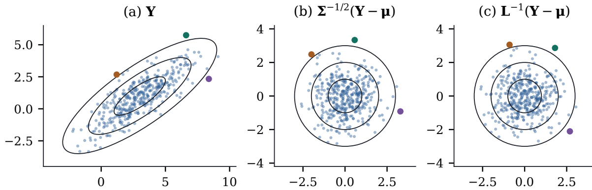
Figure 2.2.1: Whitening a correlated sample. (a) Draws with \text{Cov}(\mathbf{Y}) = \mathbf{\Sigma} and the Mahalanobis contours \Delta = 1, 2, 3 . (b) The symmetric whitening \mathbf{\Sigma}^{-1/2}(\mathbf{Y} - \boldsymbol{\mu}) . (c) The Cholesky whitening \mathbf{L}^{-1}(\mathbf{Y} - \boldsymbol{\mu}) . The contours become circles in both, and the three coloured points keep their distance from the origin. Panels (b) and (c) differ by a rotation ( Proposition 2.2.4 ).
