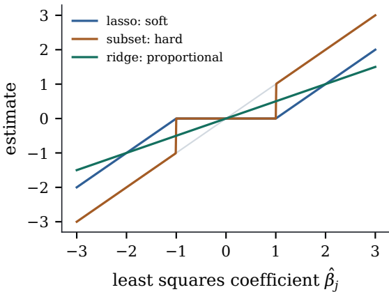
(a) orthonormal design
