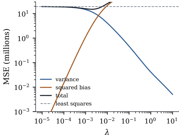
(b) MSE if the truth were the LS fit
