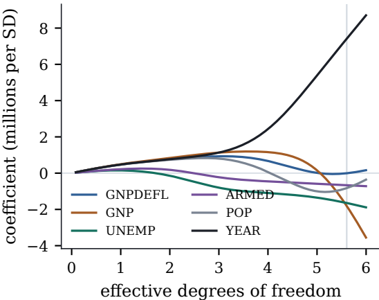
(a) ridge trace
