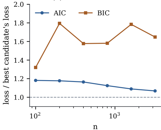
(b) no finite true model
