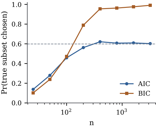
(a) a finite true model
