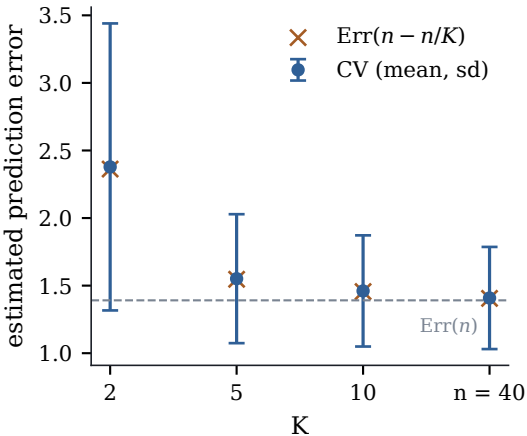
(a) bias and spread
