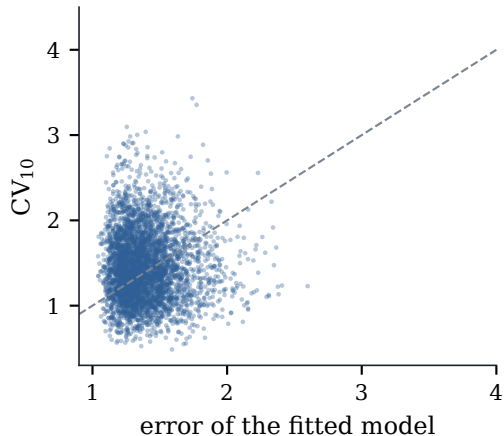
(b) what CV tracks
