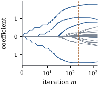
(a) path, \nu = 0.1
