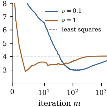
(b) test error
