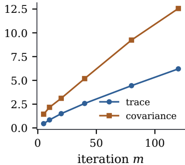
(c) degrees of freedom
