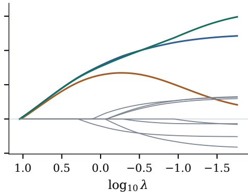
(b) elastic net, \lambda_1 = \lambda_2 = \lambda/2
