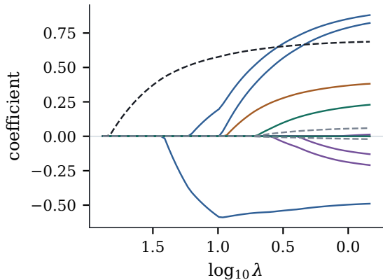
(b) lasso on indicator columns
