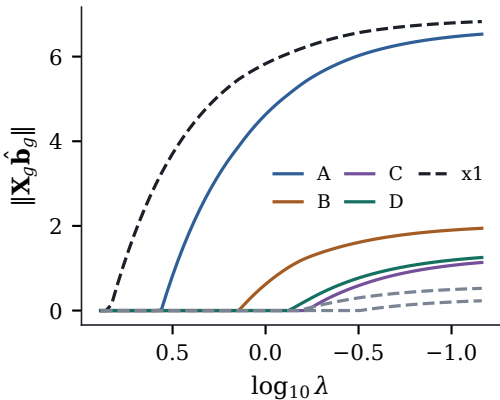
(a) group lasso: whole factors
