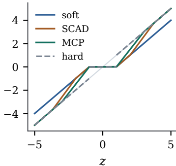
(b) thresholding rules
