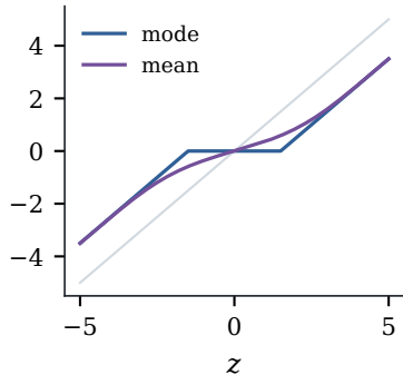
(c) Laplace prior, rate 1.5
