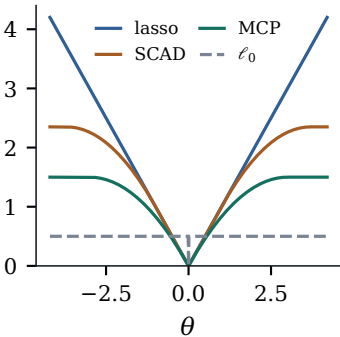
(a) penalties, \lambda = 1
