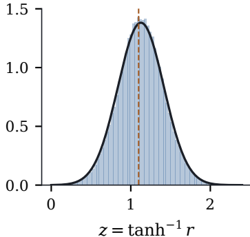
(b) Fisher's z
