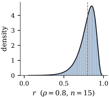
(a) exact law of r
