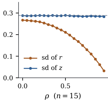
(c) variance stabilization
