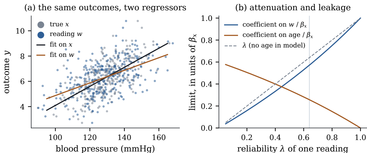
Figure 24.1.1: (a) The outcomes against true pressure (grey) and one reading (blue), with their least squares lines. (b) Limits of the coefficients of the reading and of age, in units of \beta_x , against the reliability; dashed, \lambda itself.
