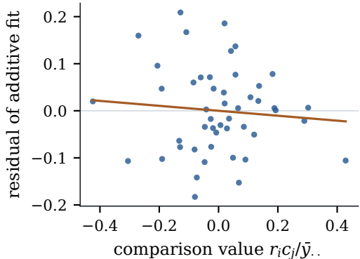
(b) log seconds: slope \hat{\theta} \bar{y}_{..} = -0.05
