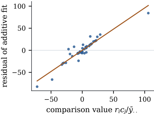
(a) seconds: slope \hat{\theta} \bar{y}_{..} = 0.96
