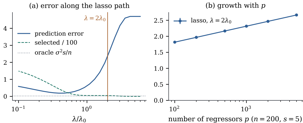
Figure 28.3.1: The lasso with n = 200 , s = 5 , \sigma = 1 . (a) Average prediction error \|\mathbf{X}(\hat{\beta}_\lambda - \beta)\|^2/n and average number of selected variables (divided by 100) along the path for p = 1000 , against \lambda/\lambda_0 . The vertical line is the theoretical choice \lambda = 2\lambda_0 , the dotted line the oracle error. (b) Prediction error at \lambda = 2\lambda_0 as p grows (logarithmic axis), with two standard errors.
