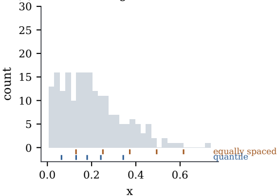
(a) a skewed design and two knot sets
