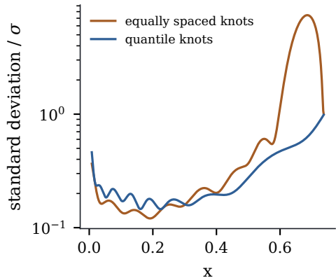
(b) pointwise variability of the fit
