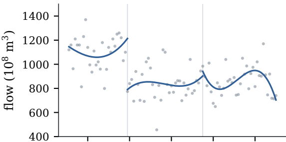
(c) continuous first derivative: 8 parameters
