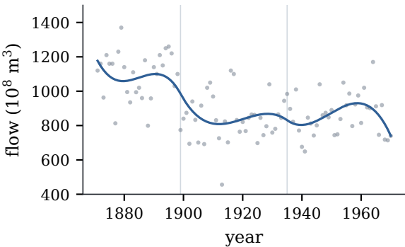
(c) continuous first derivative: 8 parameters
