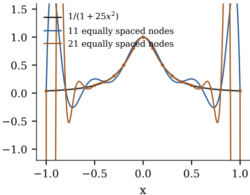
(a) Runge's phenomenon
