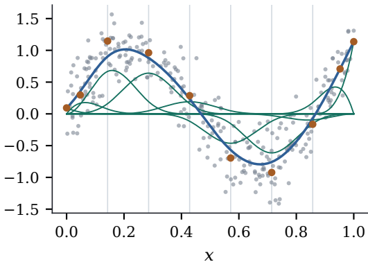
(b) the fit and its scaled basis
