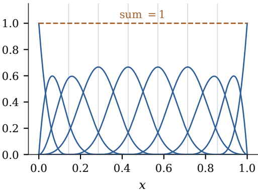
(a) cubic B-splines, 6 interior knots
