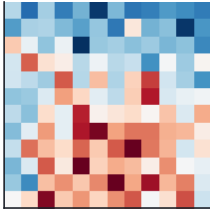
(b) unpenalized
