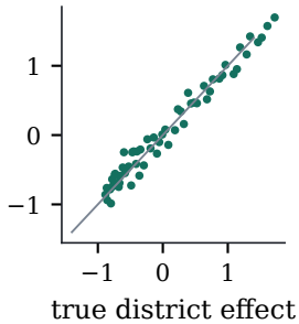
(c) spatial term
