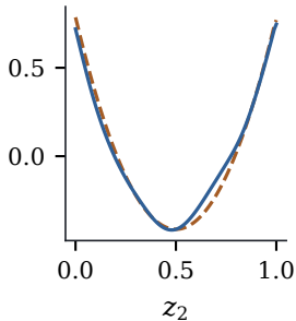
(b) varying coefficient
