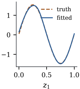
(a) smooth term
