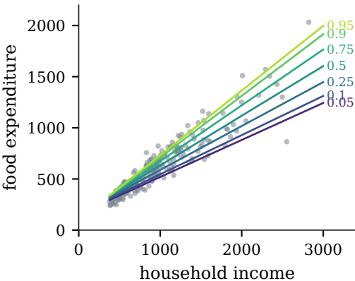
(a) seven fitted expectile lines
