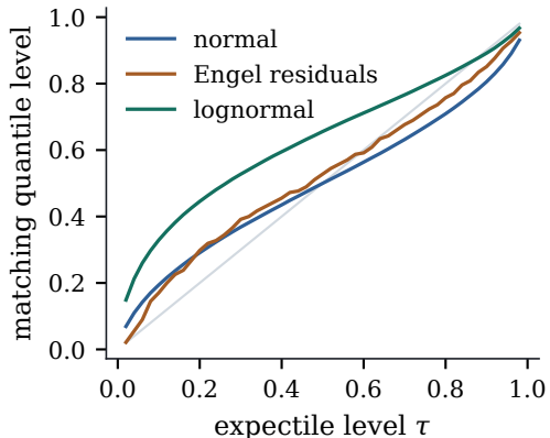
(b) the match depends on the law
