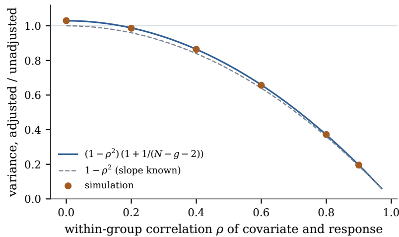
Figure 18.1.2: Variance of the adjusted difference of two group means relative to the unadjusted difference, for four groups of ten, as a function of the within-group correlation between covariate and response. The curve is Eq. 18.1.8, and the points are simulated from 100000 experiments each. The dashed curve is the ratio when the slope is known.
