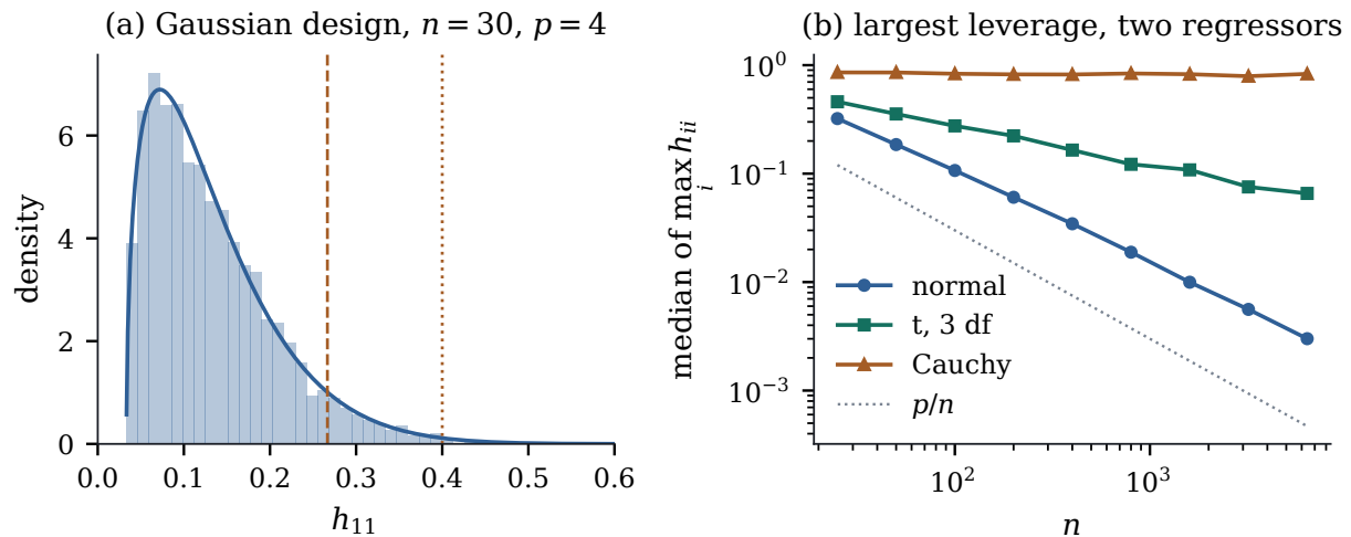
Figure 20.2.1: (a) Leverage of one case in 4000 Gaussian designs ( n = 30 , p = 4 ), the beta density of Proposition 20.2.1 , and the cut-offs 2p/n (dashed) and 3p/n (dotted). (b) Median largest leverage for normal, t_3 and Cauchy regressors.
