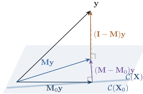
Figure 6.5.1. Nested projections. The fitted vector of the reduced model, \mathbf{M}_0 \mathbf{y} , is also the projection of \mathbf{M} \mathbf{y} onto \mathcal{C}(\mathbf{X}_0) . The three coloured pieces \mathbf{M}_0 \mathbf{y} , (\mathbf{M} - \mathbf{M}_0) \mathbf{y} and (\mathbf{I} - \mathbf{M}) \mathbf{y} are mutually orthogonal. The dashed segment is the reduced model's residual, whose squared length is the sum of the squared lengths of the two segments meeting at \mathbf{M} \mathbf{y} .
