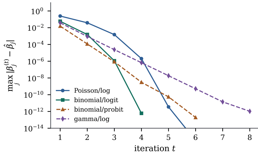
Figure 34.4.1: Convergence of iteratively reweighted least squares for four models. Solid curves are canonical links, dashed curves are not. On a logarithmic scale a quadratic rate bends downwards and a linear rate is straight.
