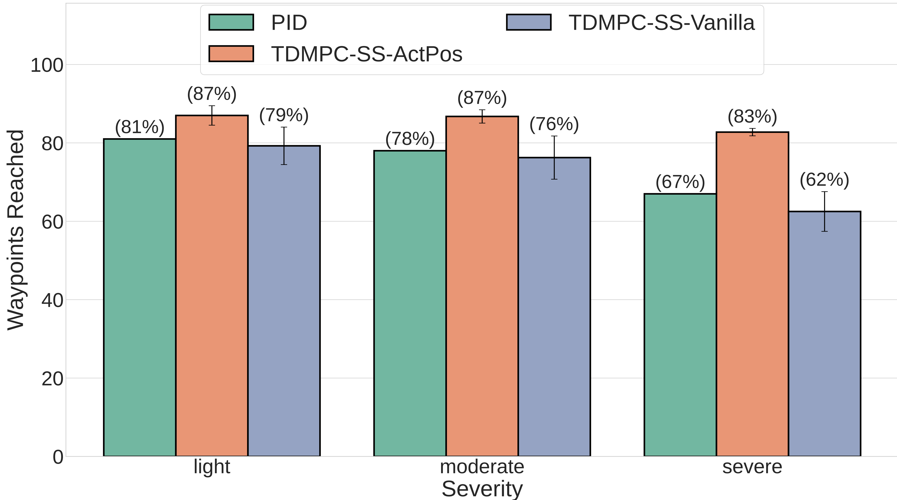
Waypoints Reached by Agent and Gusts Severity
