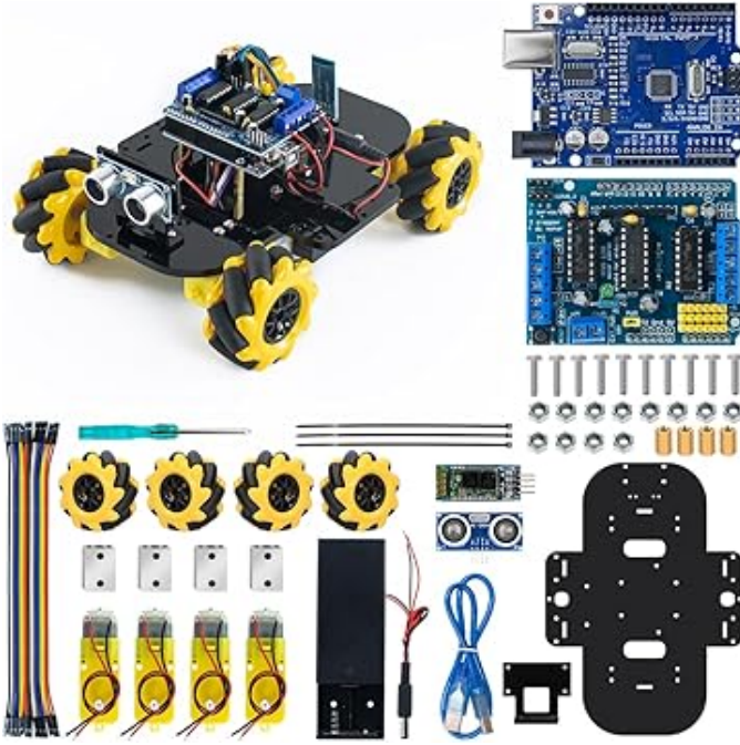
Figure 4: Amazon Swarm Kit Components: LAFVIN 4WD Mecanum Robot Car Kit Smart DIY Project Compatible with Arduino IDE.
