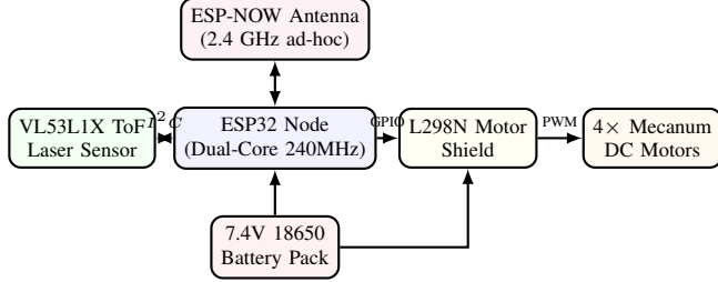
Figure 1: Decentralized ESP32 hardware schematic showing low-overhead, solderless data interfaces.
