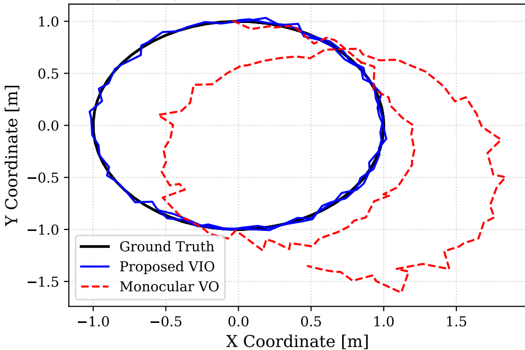
Trajectory Comparison on Sequence Room2
