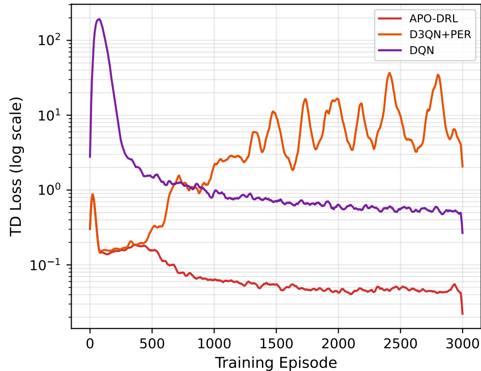
(b) TD Loss (gradient clipping L2=10)
