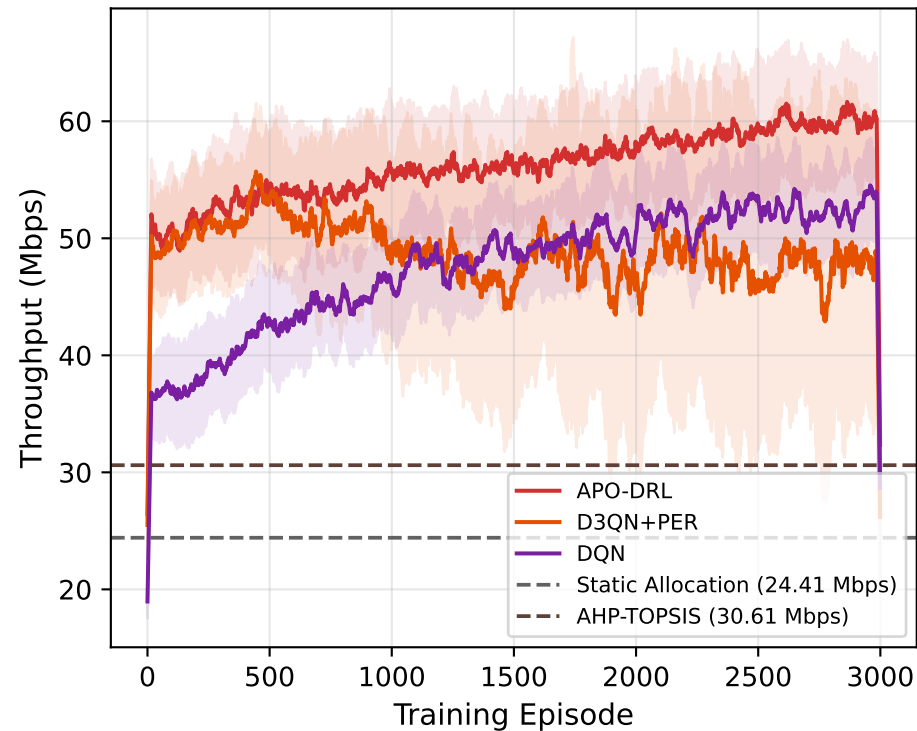
(a) Throughput Convergence ( \pm 1 std, 3 seeds)
