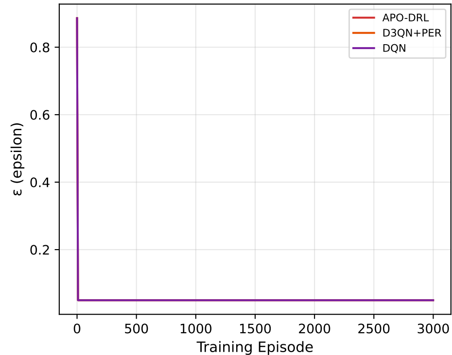
(c) Exploration Rate (identical schedule by design, min \epsilon=0.05 )
