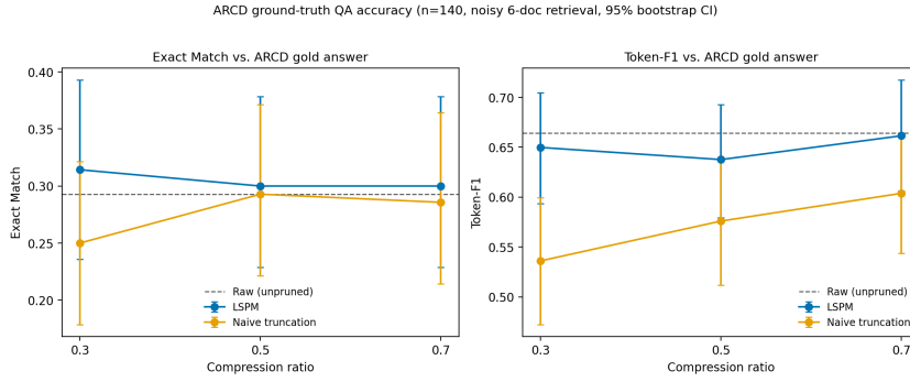
Fig. 5 two-panel plot (Exact Match, token-F1) vs. compression ratio for LSPM and naive truncation, raw/unpruned shown as a reference line, error bars showing 95% bootstrap CI
