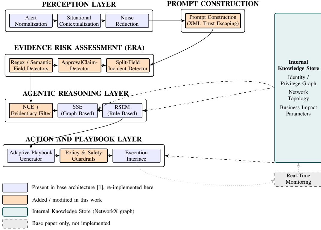
Fig. 1. Extended AgentSOC architecture mapped to this project’s module structure. Blue components are present in the base architecture [1] and re-implemented here; orange components – the Prompt Construction trust-escaping stage, the Evidence Risk Assessment layer (regex/semantic detectors, ApprovalClaimDetector, split-field detector), the NCE evidentiary threshold filter, and the policy guardrails – are the additions evaluated in this paper. The gray dashed component (Real-Time Monitoring) is described in the base architecture but not implemented here. Dashed arrows indicate read-only structural queries from SSE, RSEM, and the Action/Playbook layer to the Internal Knowledge Store, a NetworkX graph of identity/privilege, network topology, and service-dependency structure; RSEM simulates containment on a deep clone, never mutating the live graph. NCE, ERA, and Prompt Construction have no access to the Knowledge Store. The Perception Layer’s Situational Contextualization component reads the flat InMemoryKnowledgeStore for ImmutableContext facts (user role, asset criticality). The evaluation harness (Section V) constructs NCE input directly and does not invoke PerceptionPipeline or Contextualizer; the flat InMemoryKnowledgeStore therefore plays no role in any reported result and is exercised only in the Streamlit Live Mode demonstration.
