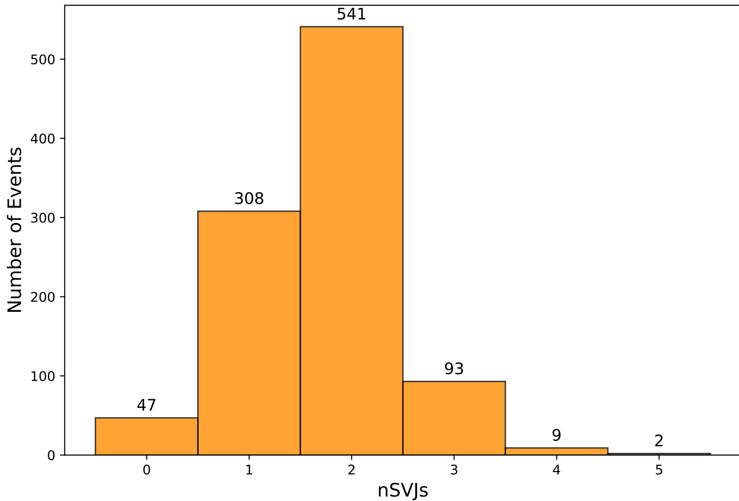
Number of Semivisible Jets (nSVJs) per Event (s-channel, M_{Z'} = 2000 GeV)
