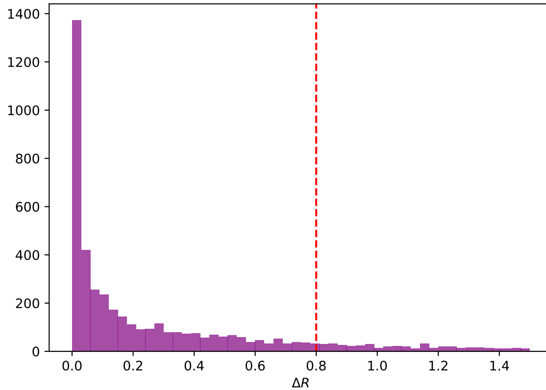
Closest GenFatJet to Dark Hadron
