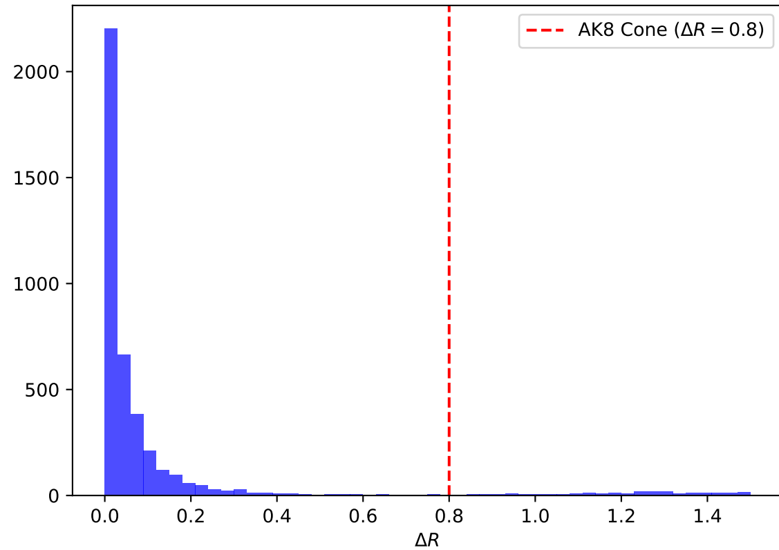
Closest Reco FatJet to GenFatJet
