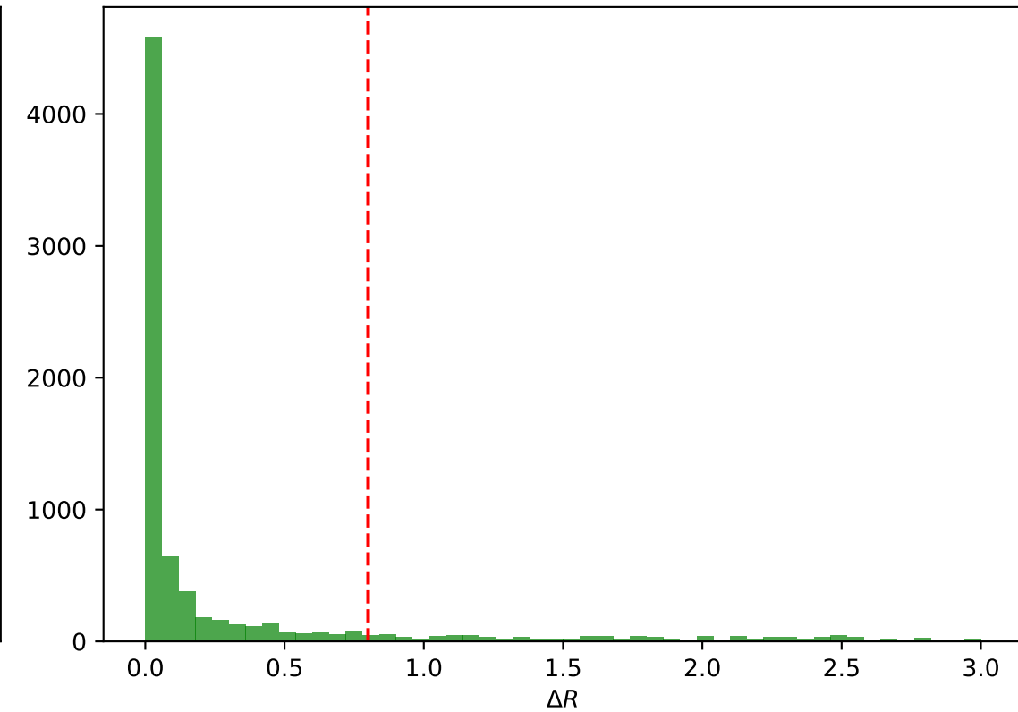
Closest Reco FatJet to Initial Dark Quark
