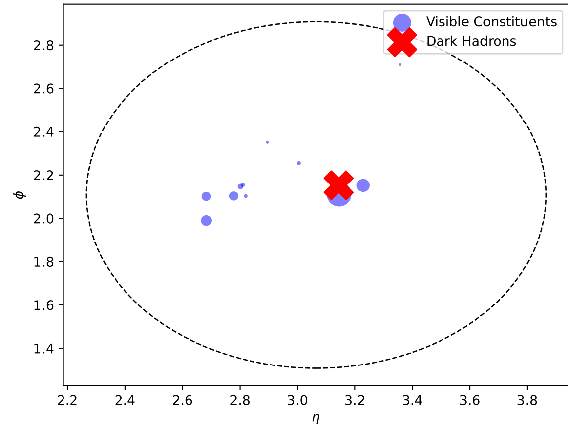
SVJ 2D Substructure Profile
