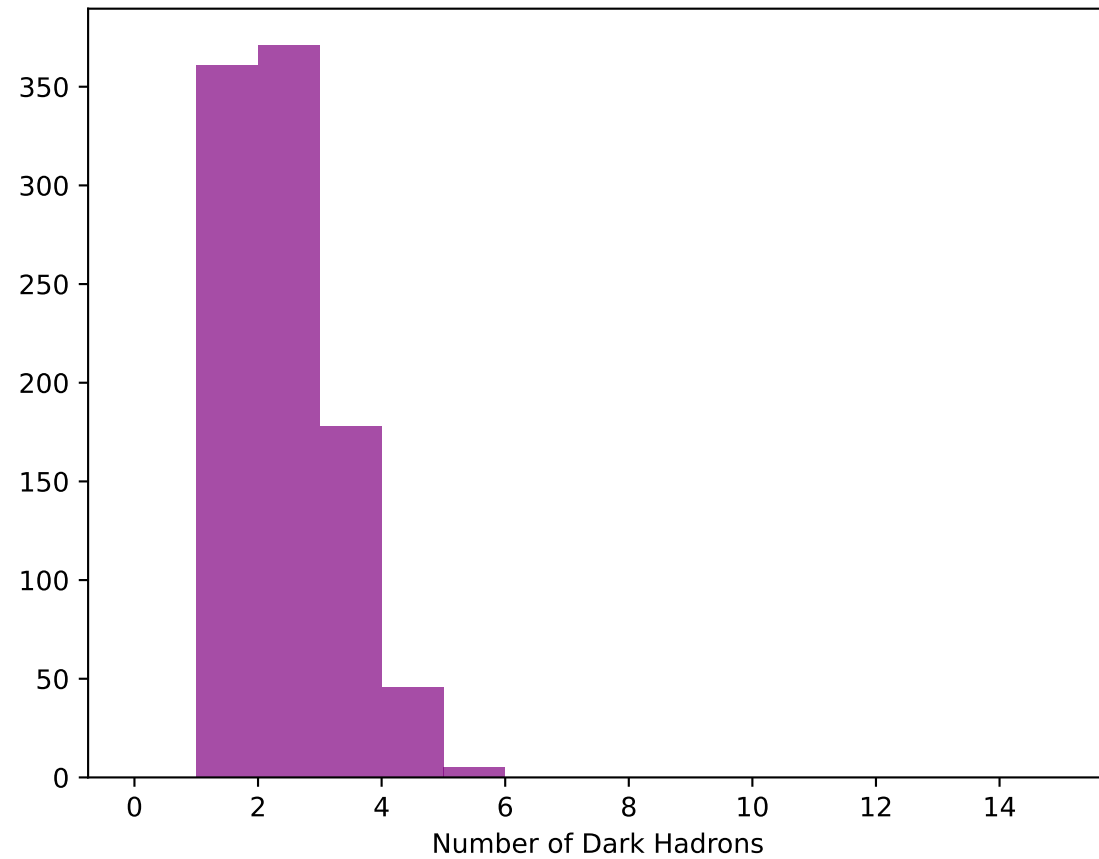
Dark Hadrons per FatJet
