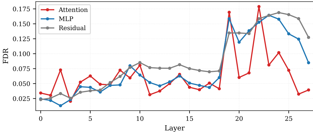
Fisher Discriminant Ratio — Raw
