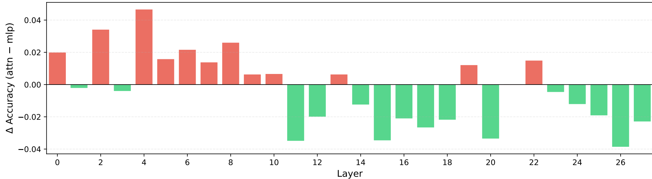
Attention – MLP Probe Accuracy (per layer) Red = attention more informative, Green = MLP more informative
