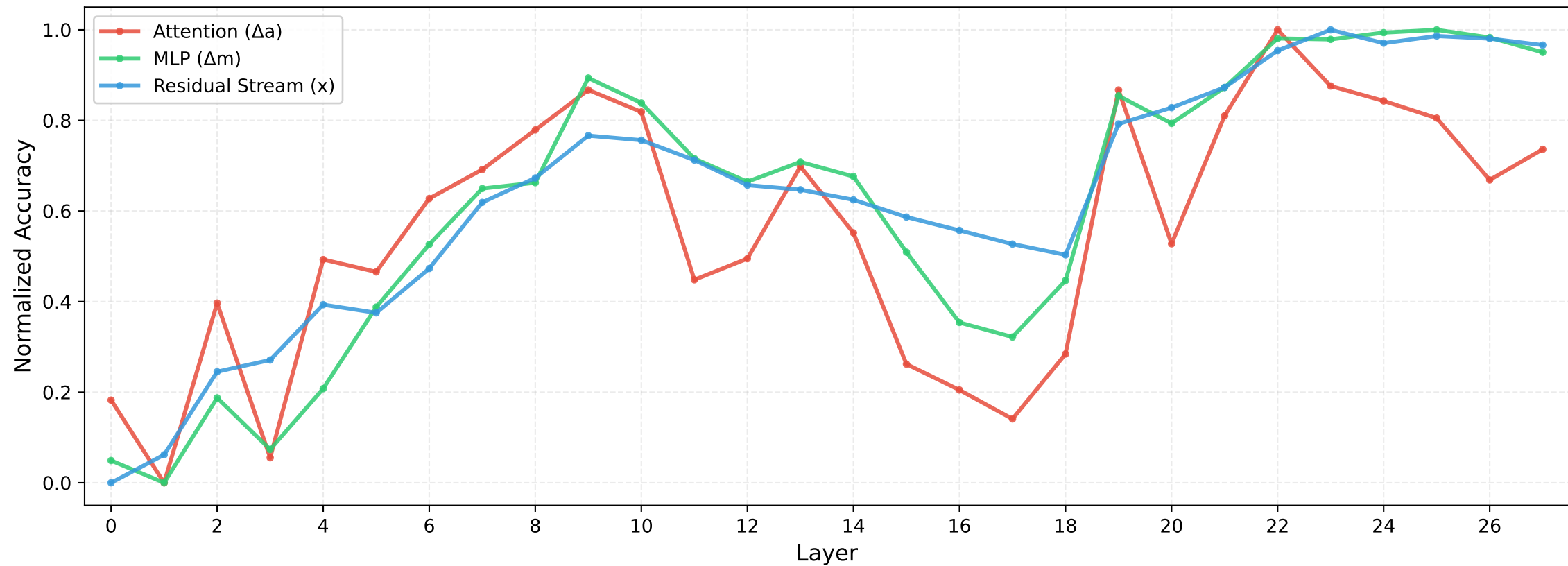
Probe Accuracy — Normalized Shape Comparison Each curve min-max normalized to [0,1] to compare layer profiles
