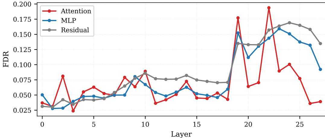
Fisher Discriminant Ratio — Normalized
