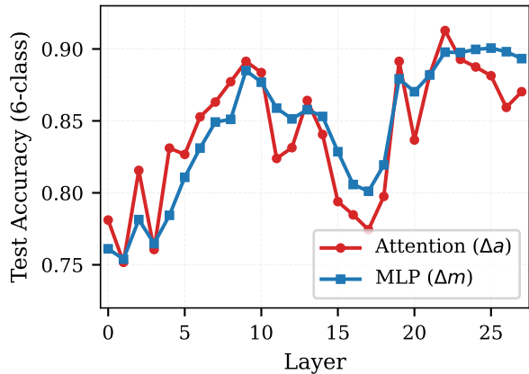
(a) Linear Probe Accuracy
