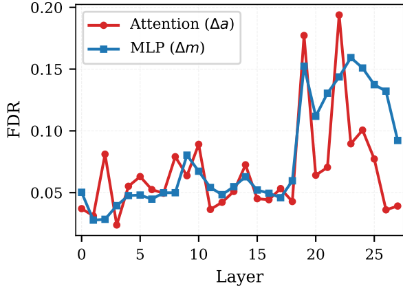
(b) Fisher Discriminant Ratio
