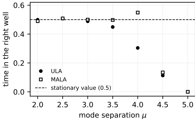
All chains started in the left well
