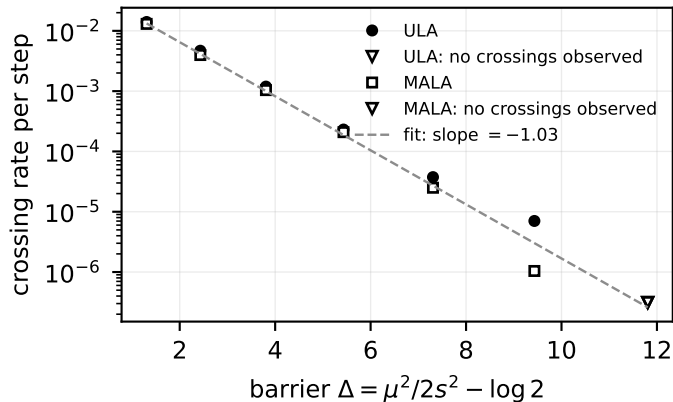
Mixing is exponential in the barrier
