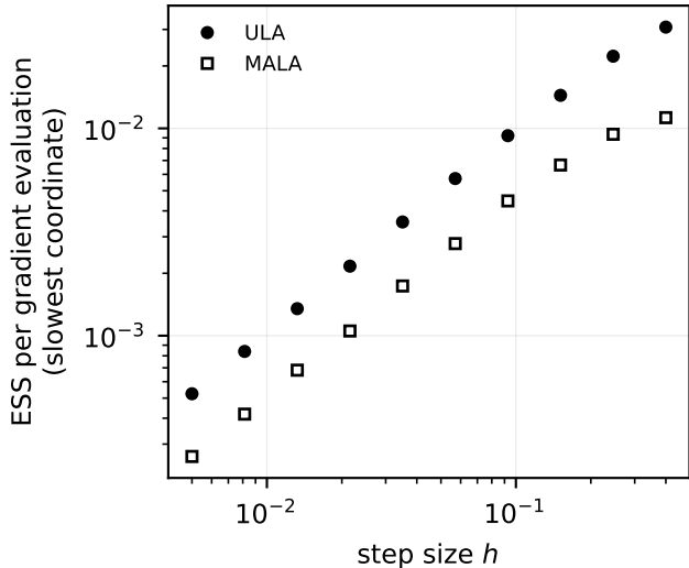
Sampling efficiency
