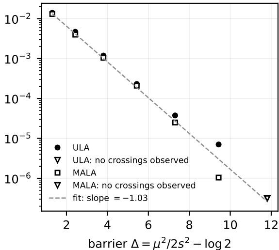
Mixing is exponential in the barrier
